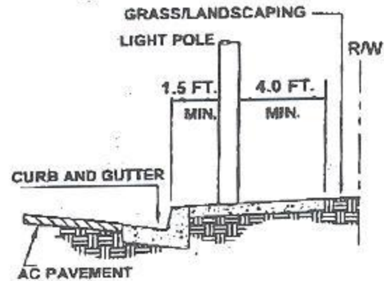
SIDEWALK ADJACENT TO CURB INSTALL 6/8 FT. MAST ARM (SEE TABLE)
